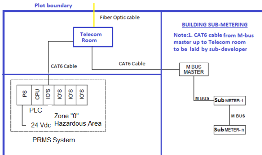
Figure 1: Gas sub-metering system
